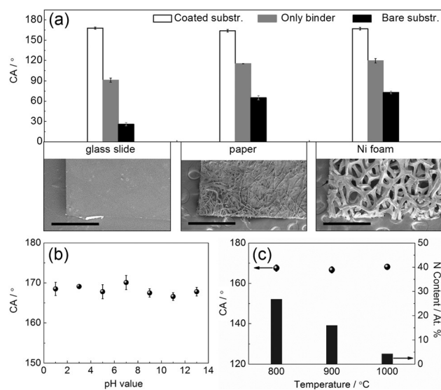
Figure 2. a) The CAs of various substrates (glass slides, paper, and Ni foam) coated with Gr-ink or with the binder (Nafion) only and of the bare substrates. Scale bar: 500 \mu\text{m} . b) Dependence of the CA of the Gr-ink-coated glass slide on the pH value. c) The CAs of glass slides coated with Gr-ink that were prepared at different temperatures and thus differ in their nitrogen content.
